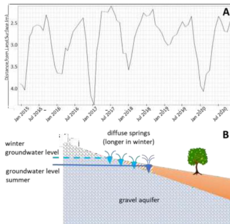
Figure 11. (A) Representative data from a Hawke's Bay monitoring well showing how groundwater levels fluctuate seasonally as weather fluctuates
