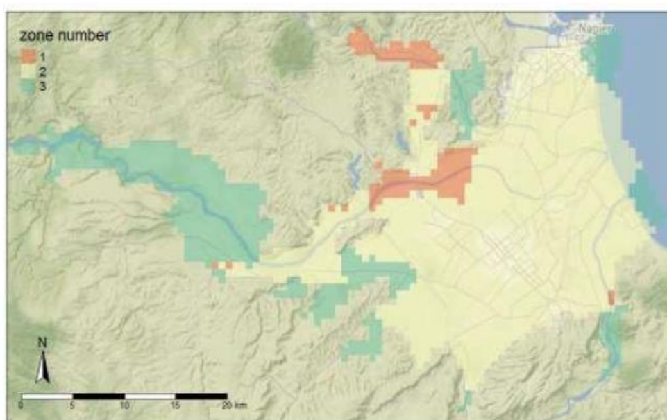
Figure 9. Map of SDZs superimposed upon a map of the Heretaunga Plains. SDZ 1 (red) shows areas where groundwater pumping is highly stream depleting whereas SDZ 3 (green) comprises
