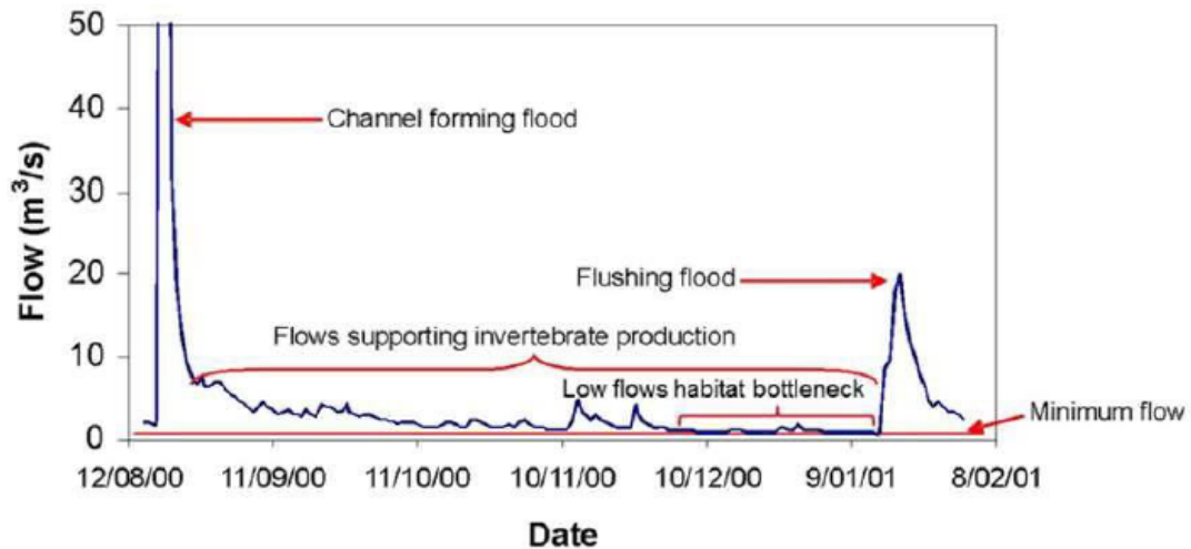
Figure 13. Schematic showing the various ecologically relevant flows.
