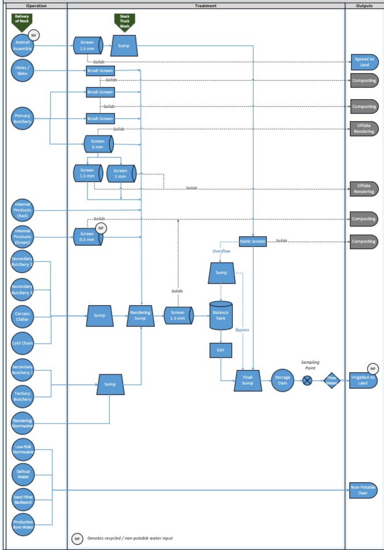
Takapau Wastewater Flow Diagram
